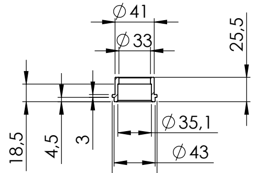
S.S. Bushing P/N 204833
