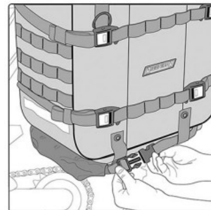
9. Connect side straps as shown
