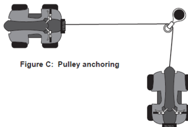
Figure C: pulley anchoring
