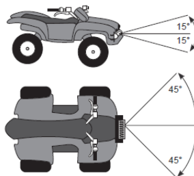
Figure B: Roller fairlead Maximum Winching Angles
