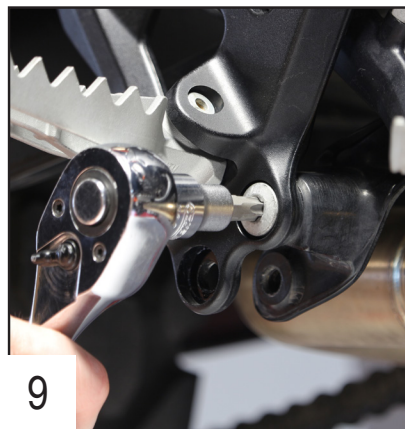
9 Untight the OEM screw, without removing it completely.
