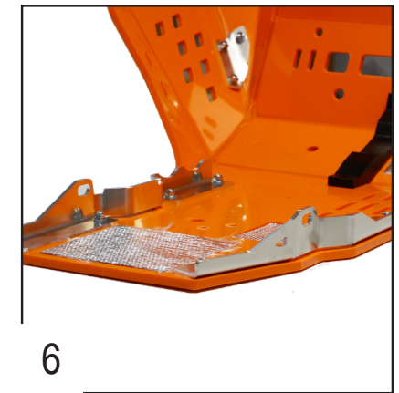
Fix the alloy parts on each side of the skid plate using 4 TFHC 6x20mm screws + M6 washers and EM6F bolts.
