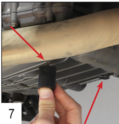
7 Screw the two silent blocks in the engine.
