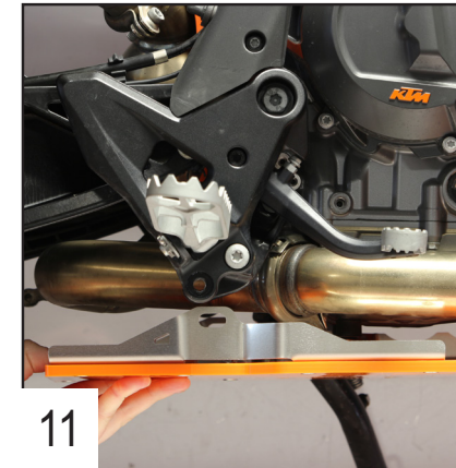
11 Lift the skid plate up to align the holes.
