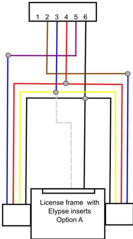
Reconfigured Setting BCM configured as "Dedicated Taillight"
