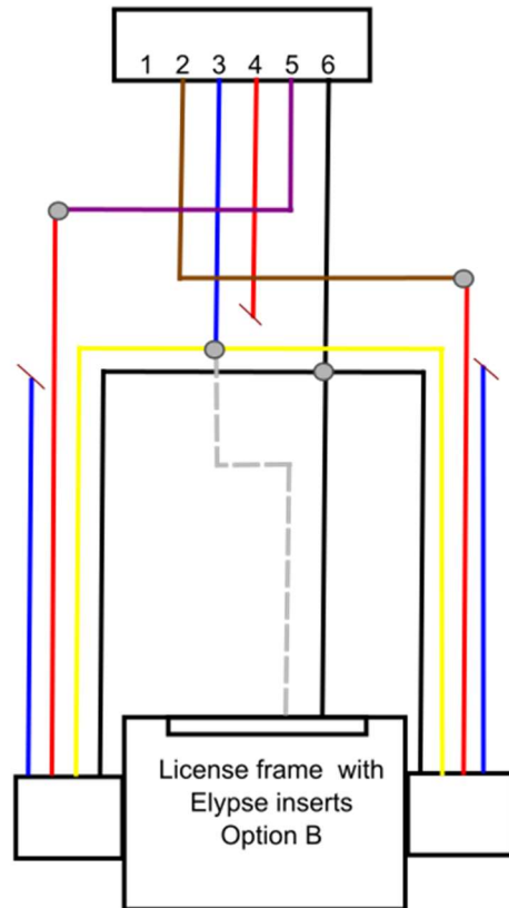
Stock Setting BCM configured as "Turn Signals Only" Blue LED wires not used, Red harness wire not used.
