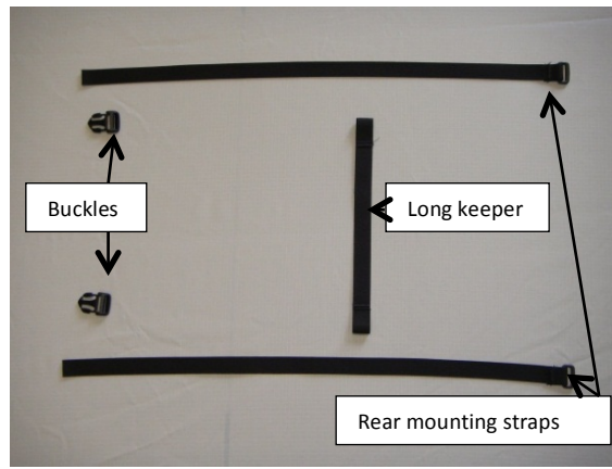
Fig.5 Rear harness
