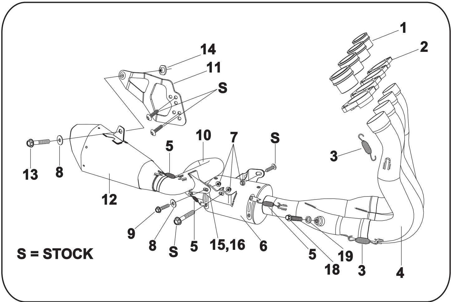
Parts Diagram
