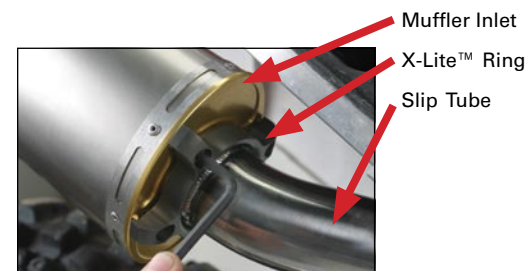
V.A.L.E.™ Assembly Detail
